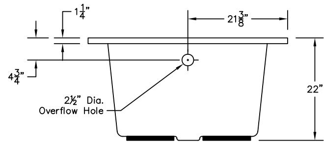
END VIEW
