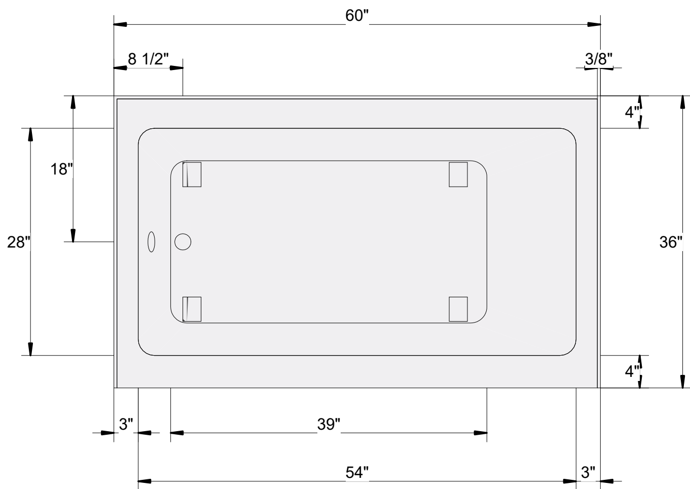
TOP VIEW
