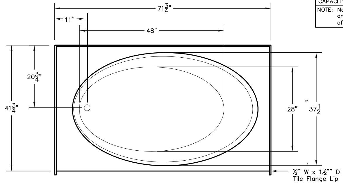
TOP VIEW
