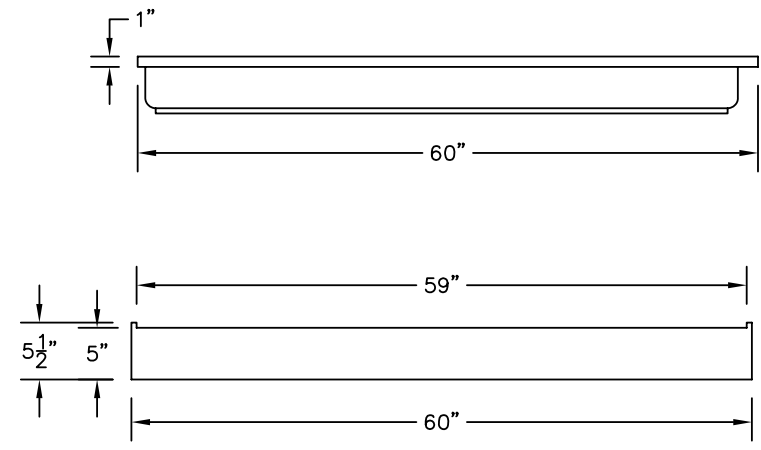
END VIEWS
